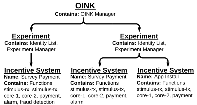
Figure 1: OINK system hierarchy. OINK sits at the highest level, followed by experiments and incentive systems. The OINK and experiment levels include managers, which provide administration, creation, and visualization at the respective level. Identity management is scoped to the experiment layer. Incentive systems are made up of multiple functions. Each function implements words from the generic incentive system vocabulary gathered from the literature. Notice that every incentive system is not the same, alarm and fraud detection functions are optional. All non-manager elements of the system run in a functions as a service (FaaS) cloud runtime.
